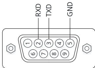
RS232 DB9 Male
